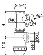
A443P: H=120-180
